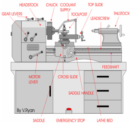
Lathe
