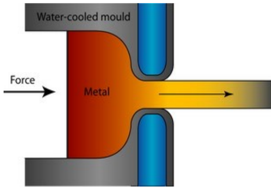
Metal Extrusion
