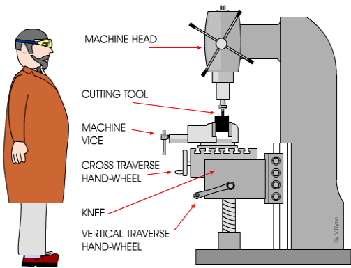
Milling Machine
