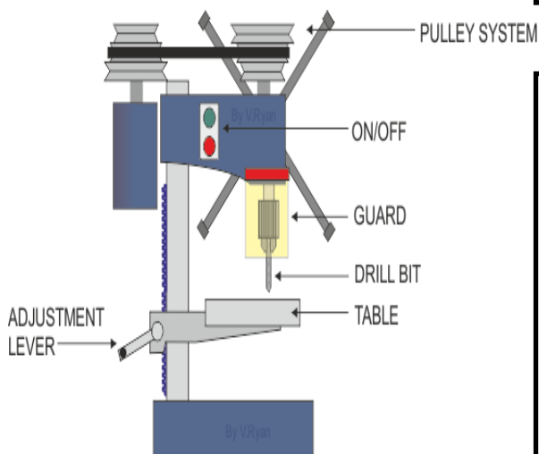
Drilling
